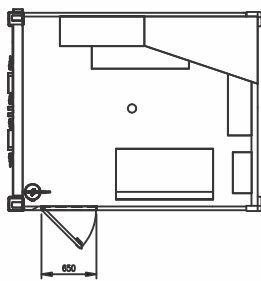
10-ft Machinery
